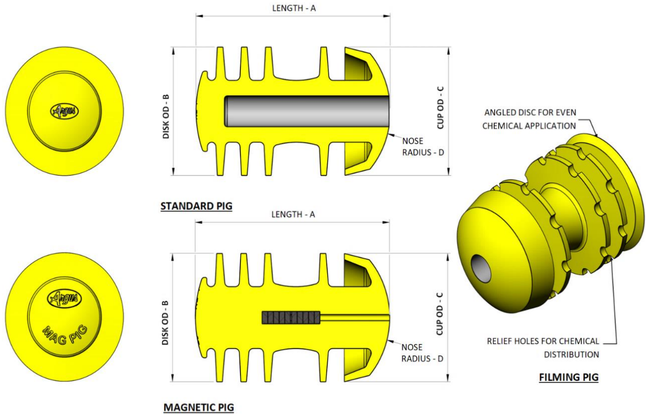
Figure 1.0: Argus Pig Dimensions
